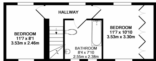
1ST FLOOR APPROX. FLOOR AREA 348 SQ.FT. (32.3 SQ.M.)
