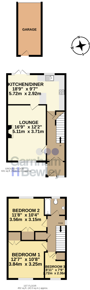
8 Warburton Close - Floorplan
