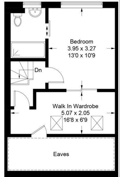
Second Floor
