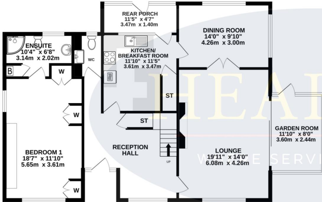
GROUND FLOOR 1183 sq.ft. (109.9 sq.m.) approx.
