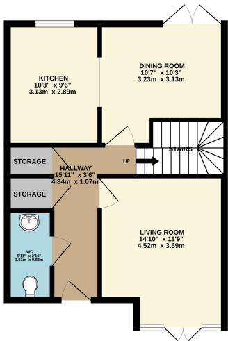
GROUND FLOOR 450 sq.ft. (41.8 sq.m.) approx.
