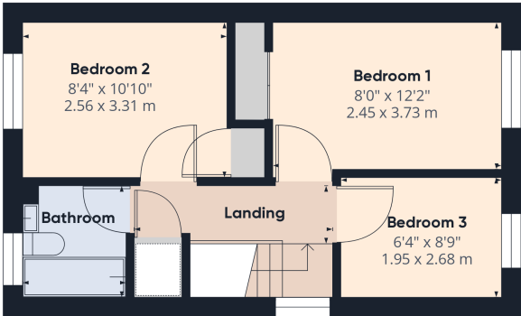
Floor 1
