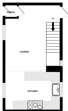
GROUND FLOOR 287 sq.ft. (26.7 sq.m.) approx.
