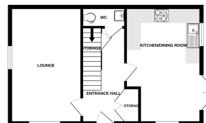
GROUND FLOOR 447 sq. ft. (41.5 sq.m.) approx.
