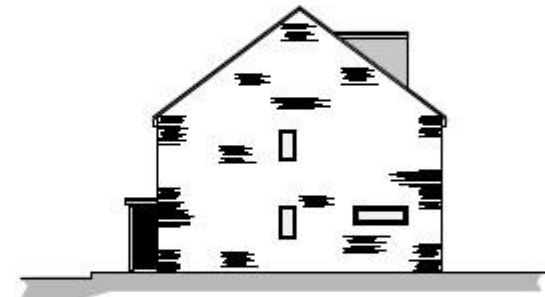
South Elevation 1:100
