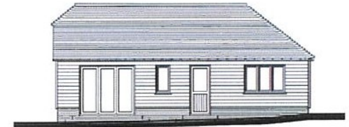
Proposed South West Elevation Scale 1:100
