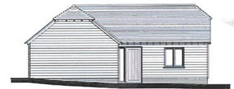
Proposed North East Elevation Scale 1:100
