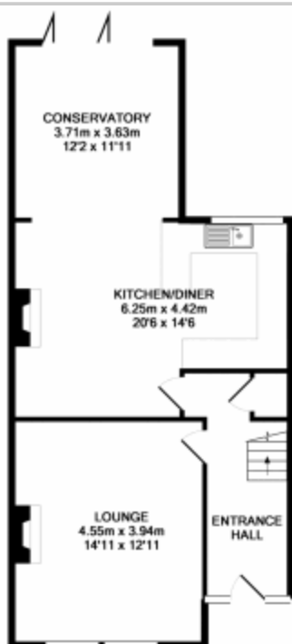
GROUND FLOOR APPROX. FLOOR AREA 99.5 SQ. M. (641 SQ. FT.)
