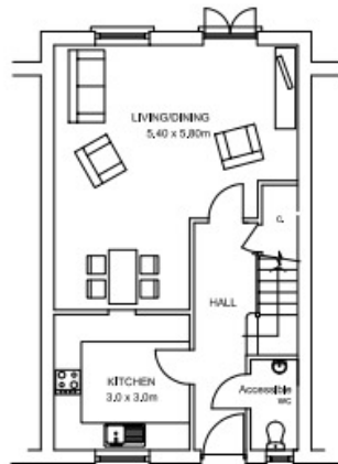
GROUND FLOOR PLAN 48.5 sq.m.
