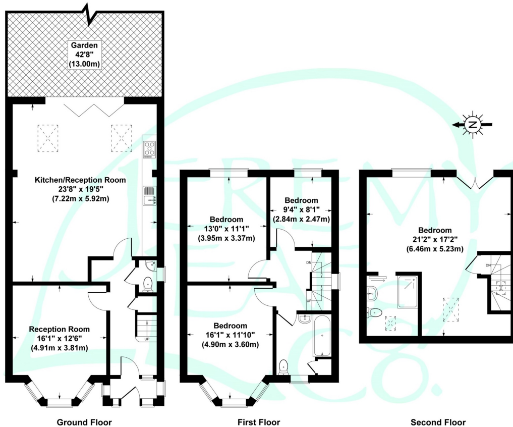
Summerlee Avenue, London, N2 Gross Internal Area 1668 sq ft / 155 sq metres Not to Scale, Produced by The Plan Portal 2021 For Illustrative Purposes Only.
